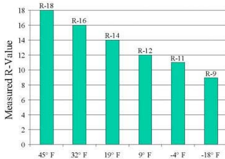
R-Value vs. Temperature For Loose-Fill Fiberglass
